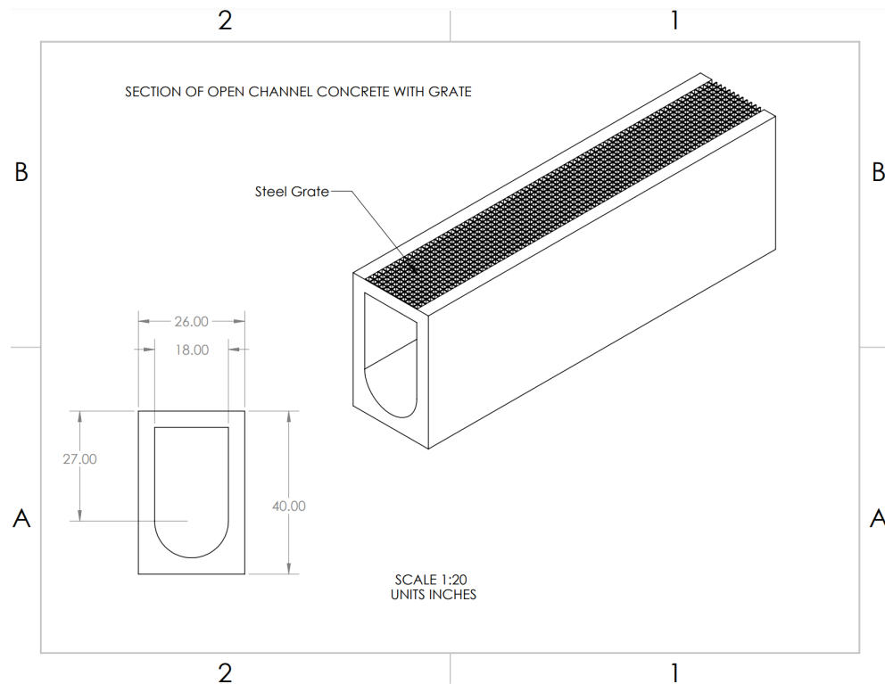
Figure 6: Cross Section of Open Channel Concrete
