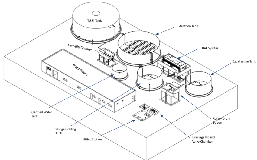
Figure 4: CAD Drawing of Stormwater Treatment Plant
