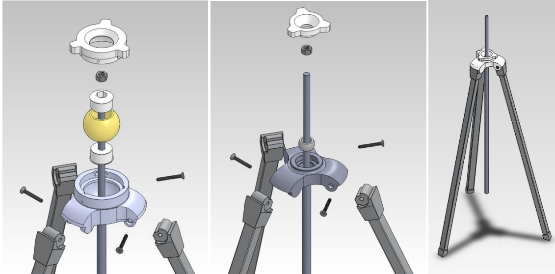
Figure 4: CAD Images of the Self-Leveling Base
