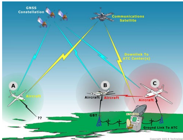
Figure 3.1: Overview of ADS-B
