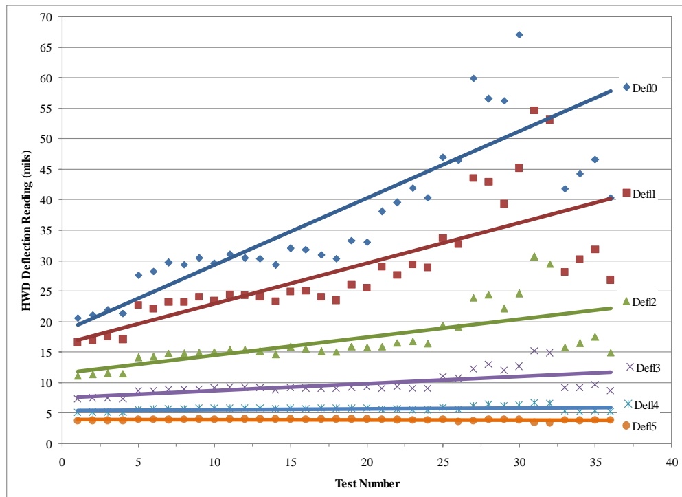
Figure 30: General HWD Deflection Response for MFC Section
