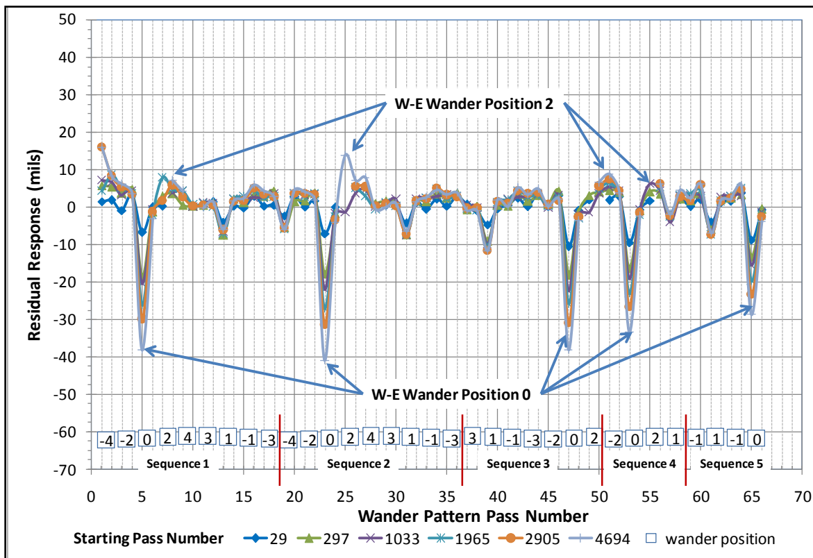
Figure 22. P209 residual response - 66 pass wander pattern and wander sequence, MFC section, B777 lane (1mil = 0.001in = 0.0254mm)
