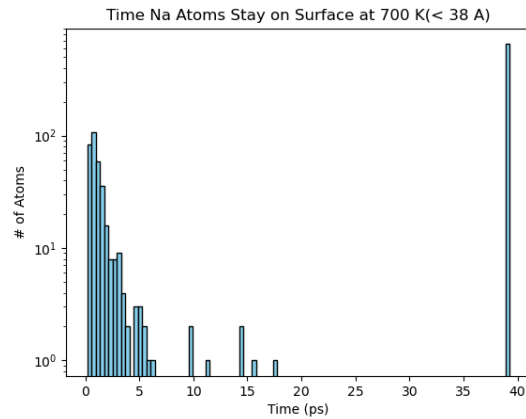
Figure 9 Residence time of sodium on the surface at 700 K. A total of 34.9% of deposited Na desorbed from the surface. The average residence time is 1.419 ps for all desorbing particles.
