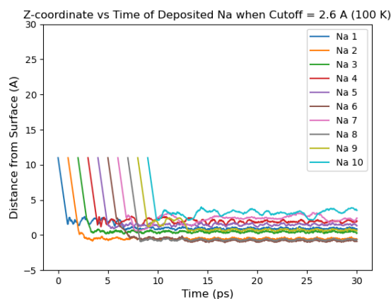
Figure 3 Vertical position of ten deposited Na atoms when surface is heated to 100 K. All atoms remain on the surface after 30 ps.
