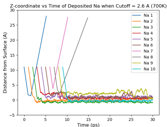
Figure 6 Vertical position of ten deposited Na atoms when surface is heated to 700 K. Three Na atoms desorbed after 30 ps had passed.
