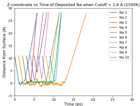
Figure 7 Vertical position of ten deposited Na atoms when surface is heated to 1500 K. All ten Na atoms desorbed after 30 ps had passed.
