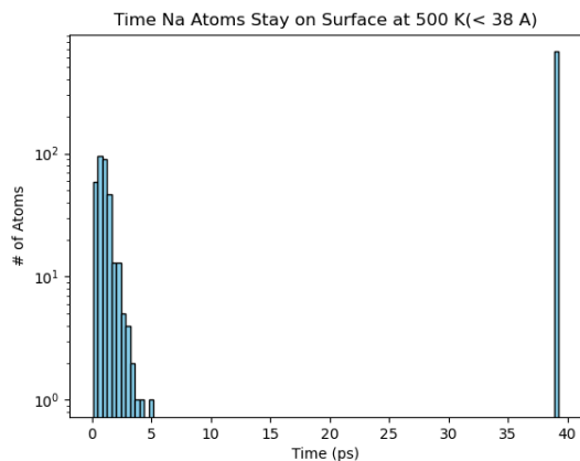
Figure 9 Residence time of sodium on the surface at 500 K. A total of 33.2% of deposited Na desorbed from the surface. The average residence time is 1.030 ps for all desorbing particles.
