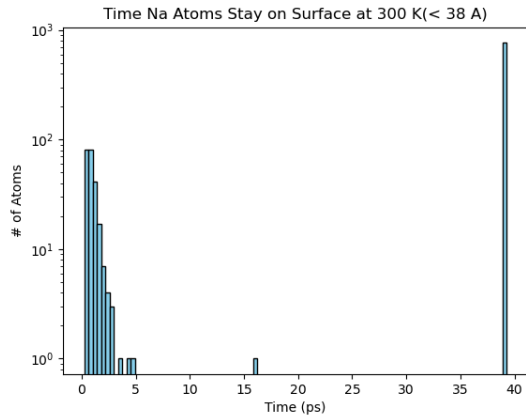
Figure 8 Residence time of sodium on the surface at 300 K. A total of 23.8% of deposited Na desorbed from the surface. The average residence time is 0.982 ps for all desorbing particles.
