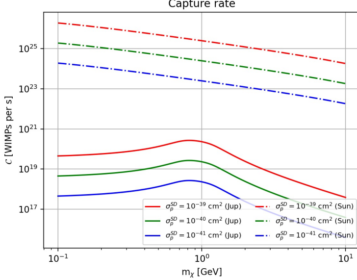
Figure 1: Capture rate of WIMPs in both Jupiter and the Sun. The resonance peak at roughly 1 GeV corresponds to the WIMP mass being closely matched to the target. This effect is hardly noticeable in the Sun because of its larger escape velocity ( v_{\text{esc,S}} \simeq 10v_{\text{esc,J}} ) [5, 26].
