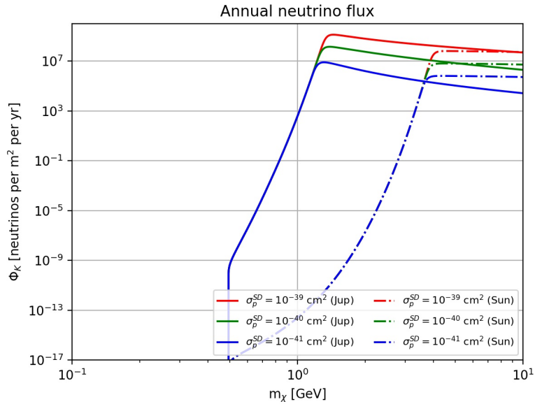
Figure 4: The dot-dashed lines give the flux of 236 MeV neutrinos at the surface of the Earth from WIMP annihilation in the Sun for three different spin-dependent cross sections. The solid lines give the flux from WIMP annihilation in Jupiter, near the surface of Jupiter. Note that the flux near Jupiter is substantially higher in the 1-4 GeV region. We have included the phase space factor of \sqrt{(1 - m_K^2/m_{WIMP}^2)} in the figure - this is negligible above 1 GeV.
