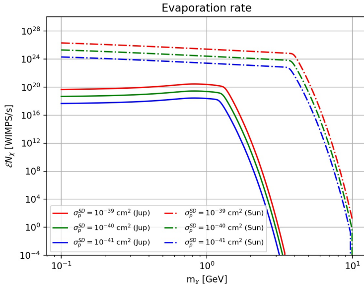
Figure 3: Evaporation of WIMPs inside Jupiter and the Sun. In both cases, we note that just above a certain mass m_{\text{evap}} evaporation drops sharply to zero, whereas below m_{\text{evap}} it is comparable to the rate of WIMPs being captured. We have estimated this mass to be about 1.3 GeV for Jupiter and 3.3 GeV for the Sun, in agreement with previous estimates [28, 6, 21, 22, 20]. This is not a great restriction on Jupiter as sub-GeV WIMPs are kinematically unable to annihilate into kaons.
