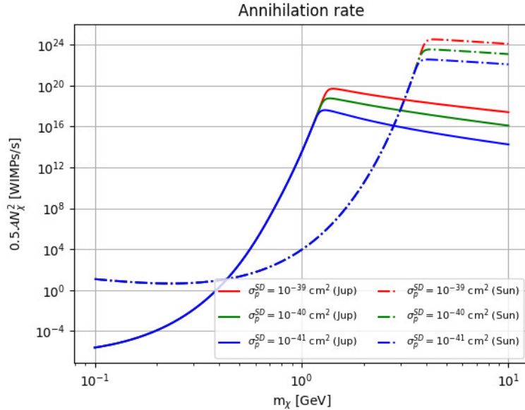
Figure 2: Annihilation of WIMPs into SM particles in Jupiter and the Sun. It should be noted that this is the total number of WIMP annihilations, but only a fraction of them produce kaons which decay into muon neutrinos. The annihilation rate is comparable to the capture rate above the evaporation mass because both Jupiter and the Sun are in equilibrium ( \tanh(t/\tau) \simeq 1 ).
