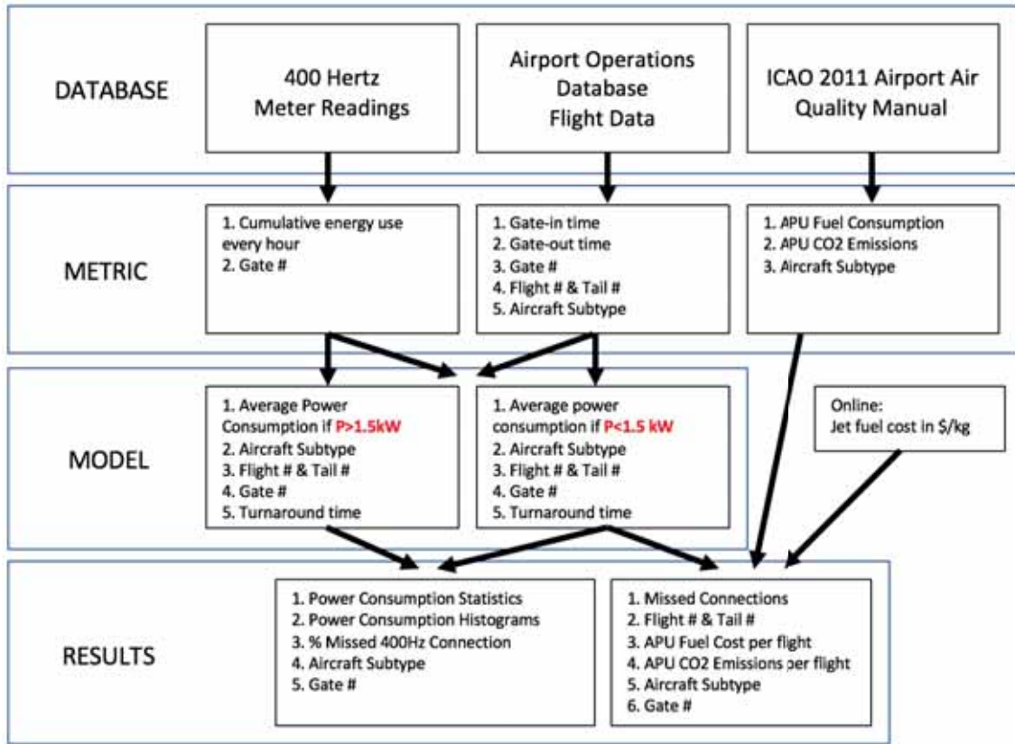
Figure 6. Database Interaction Diagram
