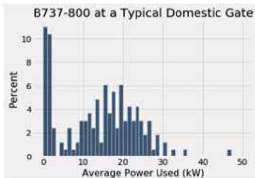
Figure 9. B737-800 at a typical domestic gate
