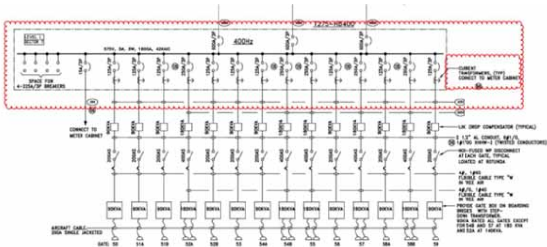
Figure 5. 400Hz Line Diagrams at SFO (Ref: SFO)
