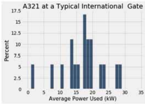
Figure 11. A321 at a typical international gate
