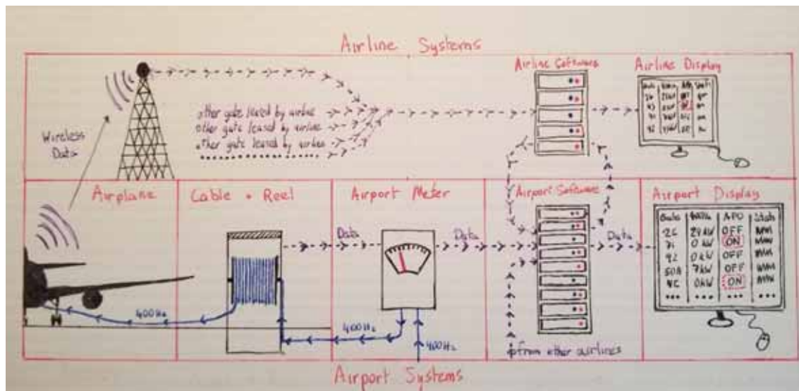
Figure 14. Proposed Collaborative System
