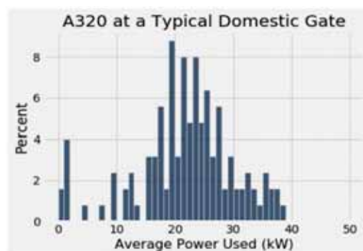
Figure 10. A320 at a typical domestic gate
