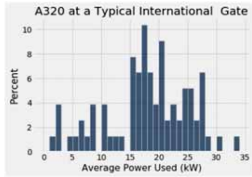
Figure 12. A320 at a typical international gate
